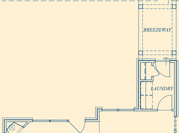
PARTIAL FIRST FLOOR PLAN W/ OPT. BREEZEWAY AND OPT. 3-CAR DETACHED GARAGE
