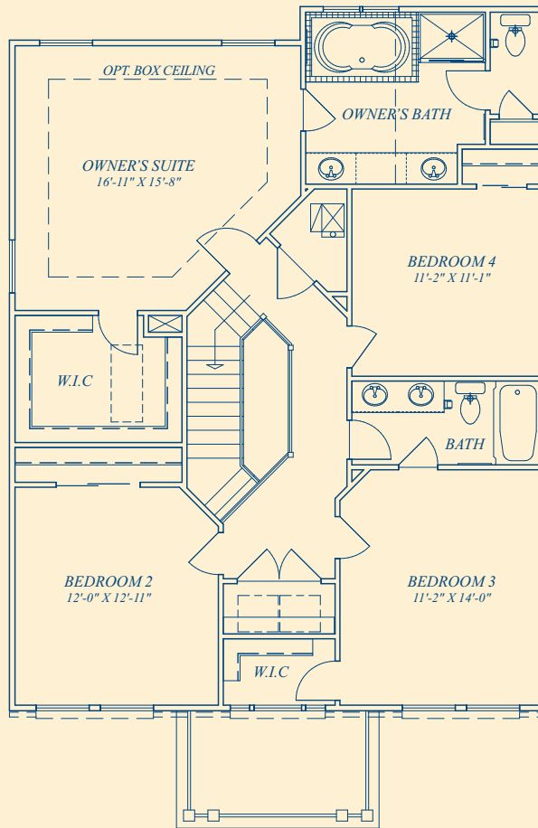
STANDARD SECOND FLOOR PLAN (SHOWN WITH ELEV. 1)
