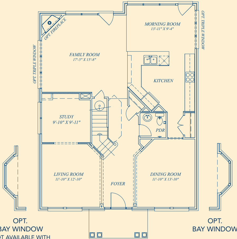
STANDARD FIRST FLOOR PLAN (SHOWN WITH ELEV. 1)
