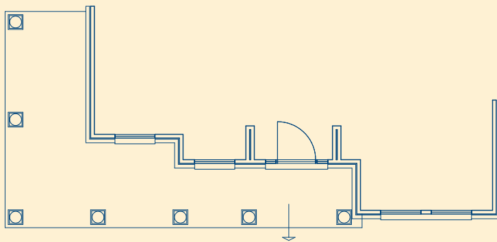
PARTIAL FIRST FLOOR PLAN WITH OPT. WRAP-AROUND PORCH (SHOWN WITH ELEV. 3)
