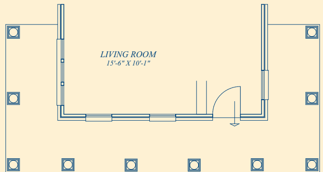
PARTIAL FIRST FLOOR PLAN WITH OPT. WRAP-AROUND PORCH (SHOWN WITH ELEV. 2, AVAILABLE WITH ELEV. 6)
