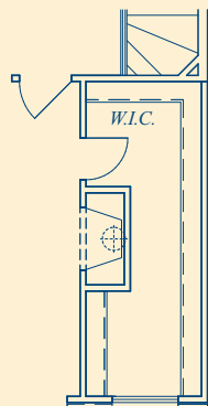
OPT. FIREPLACE WITH OPT. WALK-IN CLOSET (NOT AVAILABLE WITH LOFT)
