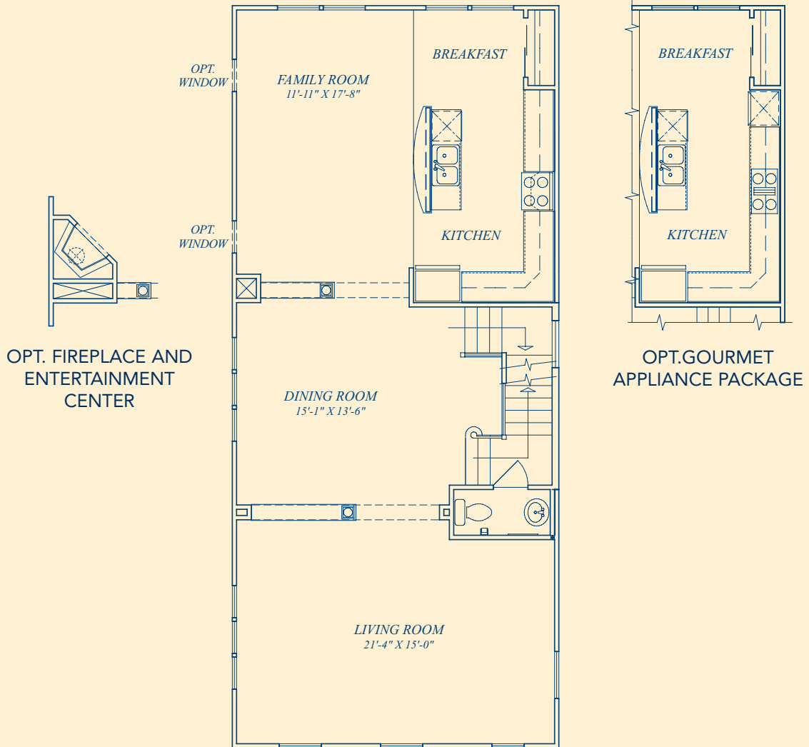
SECOND FLOOR PLAN (SHOWN WITH ELEV. 1)
