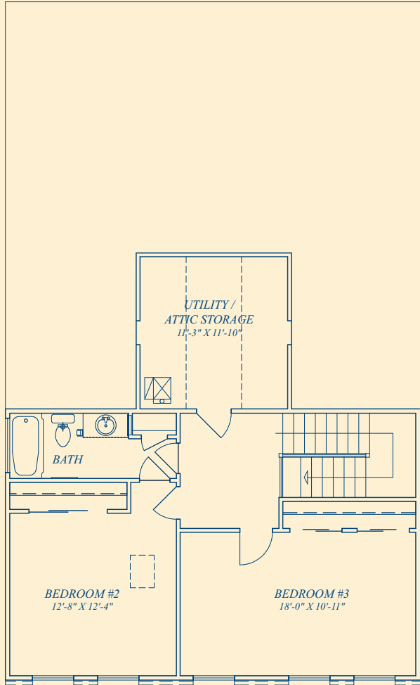
STANDARD SECOND FLOOR PLAN (SHOWN WITH ELEV. 1)
