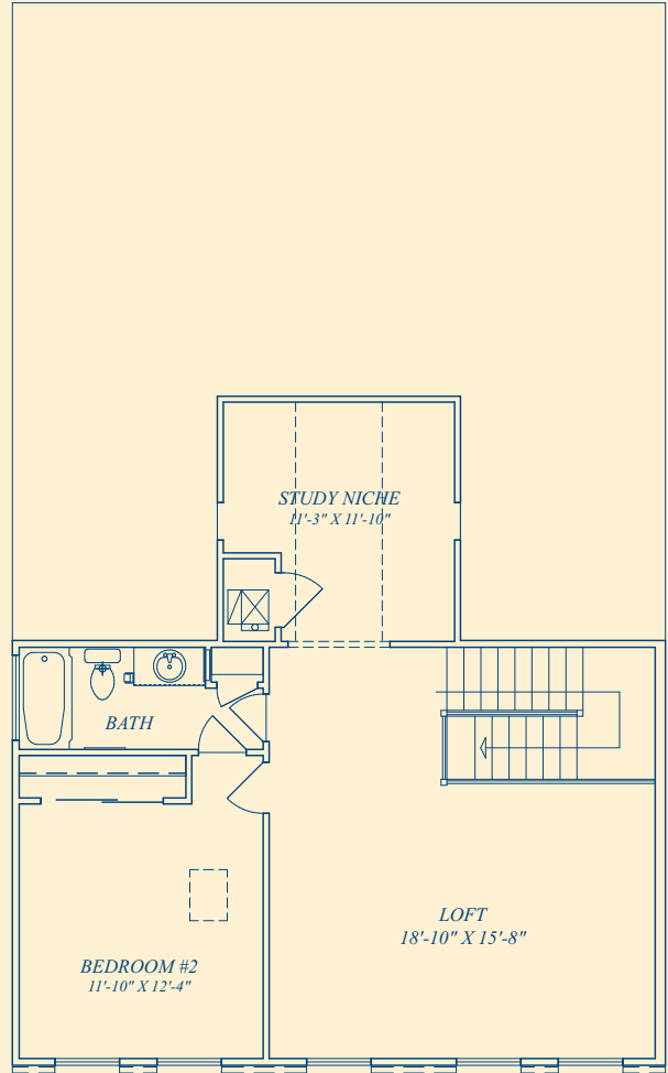
OPT. SECOND FLOOR PLAN (SHOWN WITH ELEV. 1)
