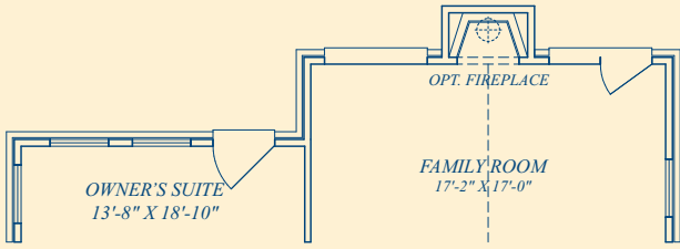
OPT. 4' REAR EXTENSION
