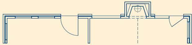
PARTIAL FIRST FLOOR PLAN W/ OPT. 3-CAR DETACHED GARAGE
